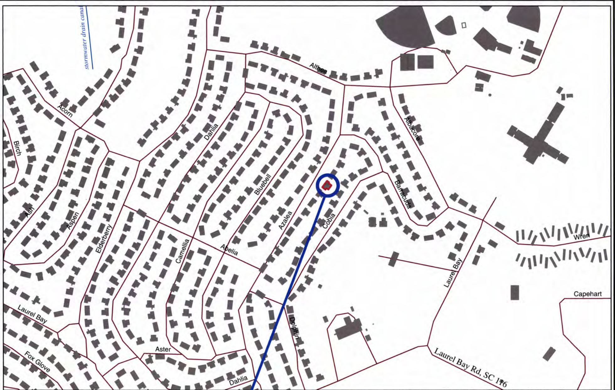
FIGURE 1: LOCATION MAP 837 AZALEA DRIVE LAUREL BAY, BEAUFORT SC
